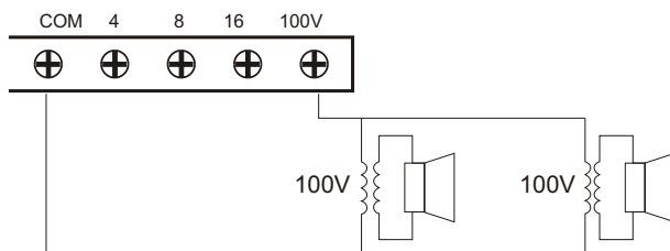
Total impedance 100V
